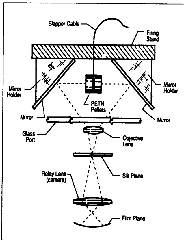
Fig. 4. Streak camera view of bidirectional assembly.
